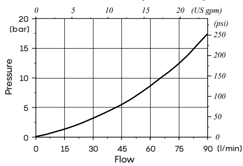
Anti-cavitation valve pressure drop
