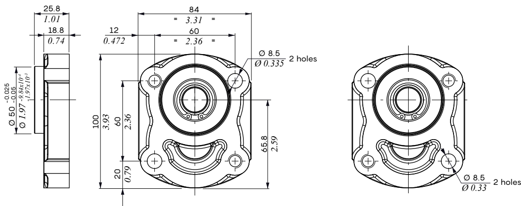
B50CX configuration
