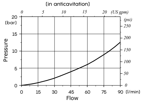
Anti-shock plus anti-cavitation valves pressure drop
