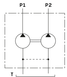
Hydraulic circuit
